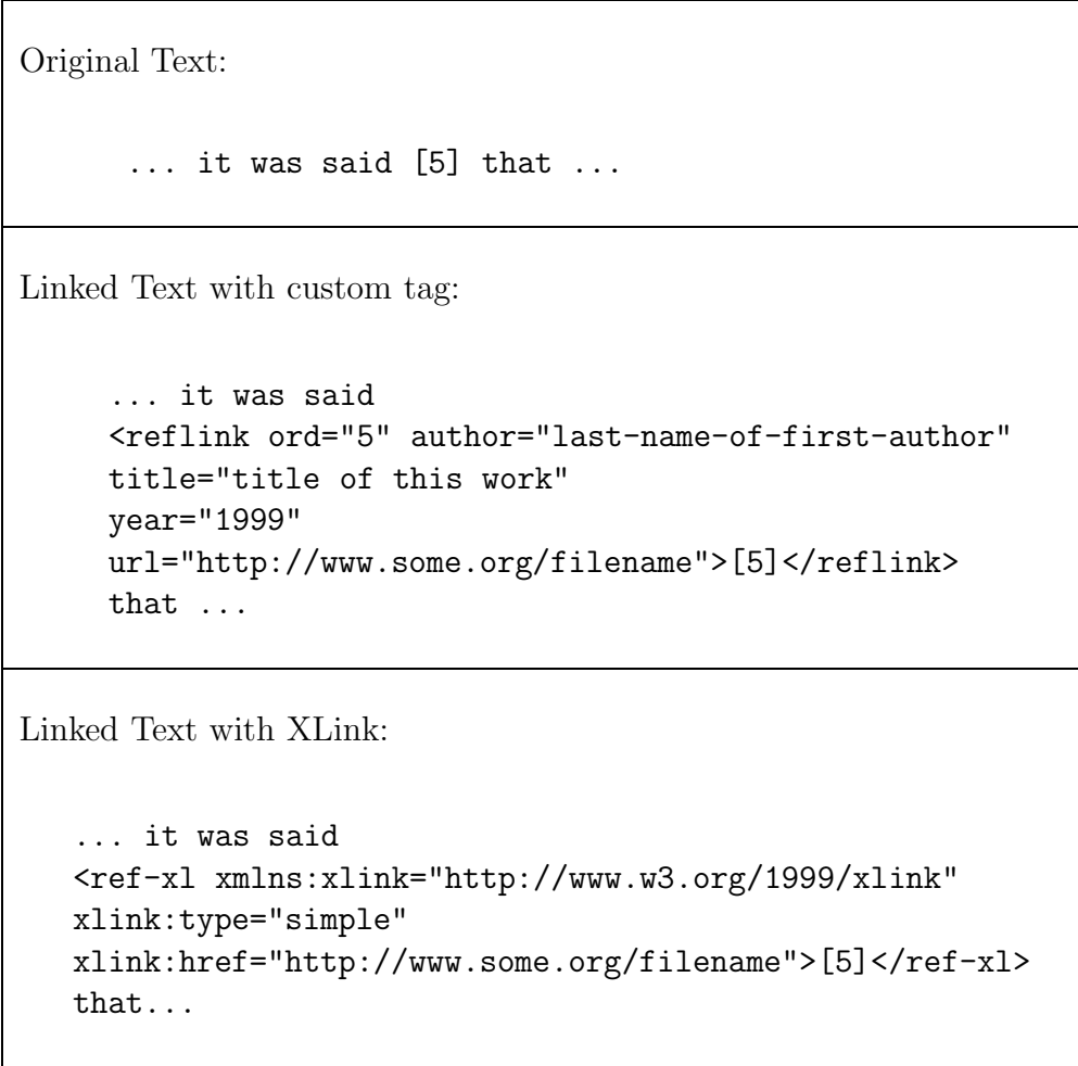
Figure 6: A linked XML Item, first with reflink then with XLink.
