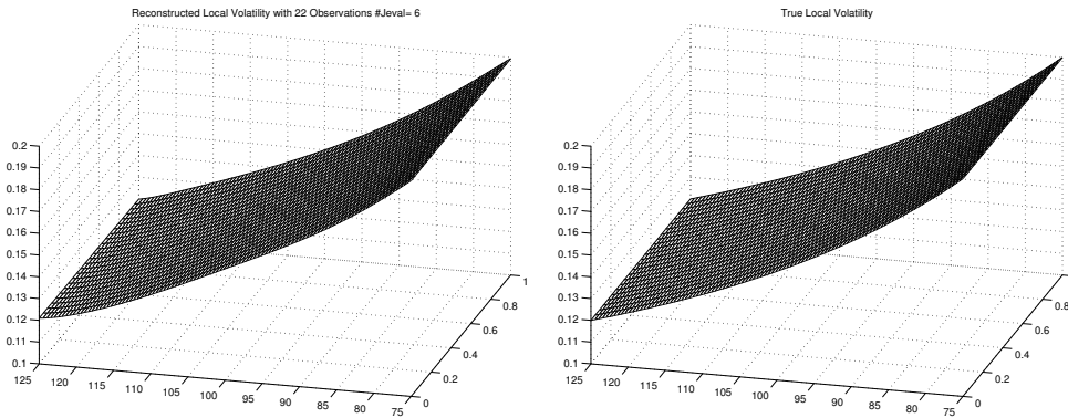
FIG. 2. The Reconstructed and True Local Volatility
