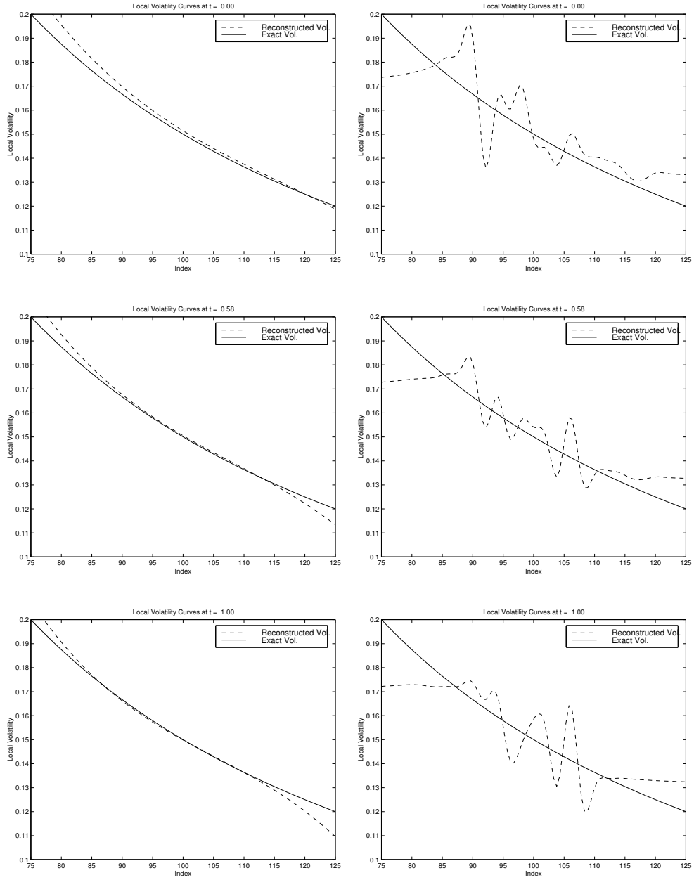
FIG. 4. Left: Knots = [.4S_{init} : .4S_{init} : 1.6S_{init}] \times [0, 1] , Right: Knots = [0 : 2 : 200] \times [0, 1]
